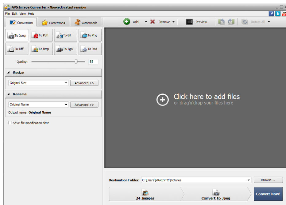
Figure 6: Start page
