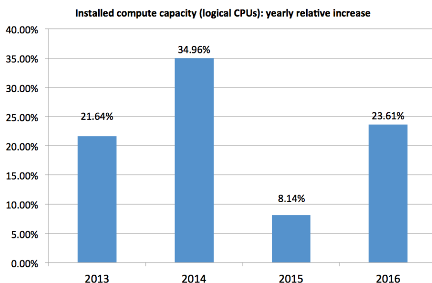
Figure 1 Yearly relative increase of the number of installed logical CPUs in the EGI HTC platform (2013-2016). As shown in this diagram, the yearly increase is very variable; however, in 2016 the relative increase shows a significant increase when compared to 2015.
