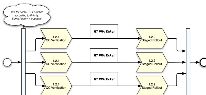
Figure 33 Software assessment
