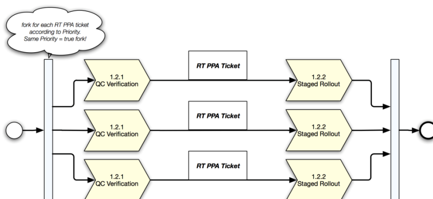
Figure 33 Software assessment
