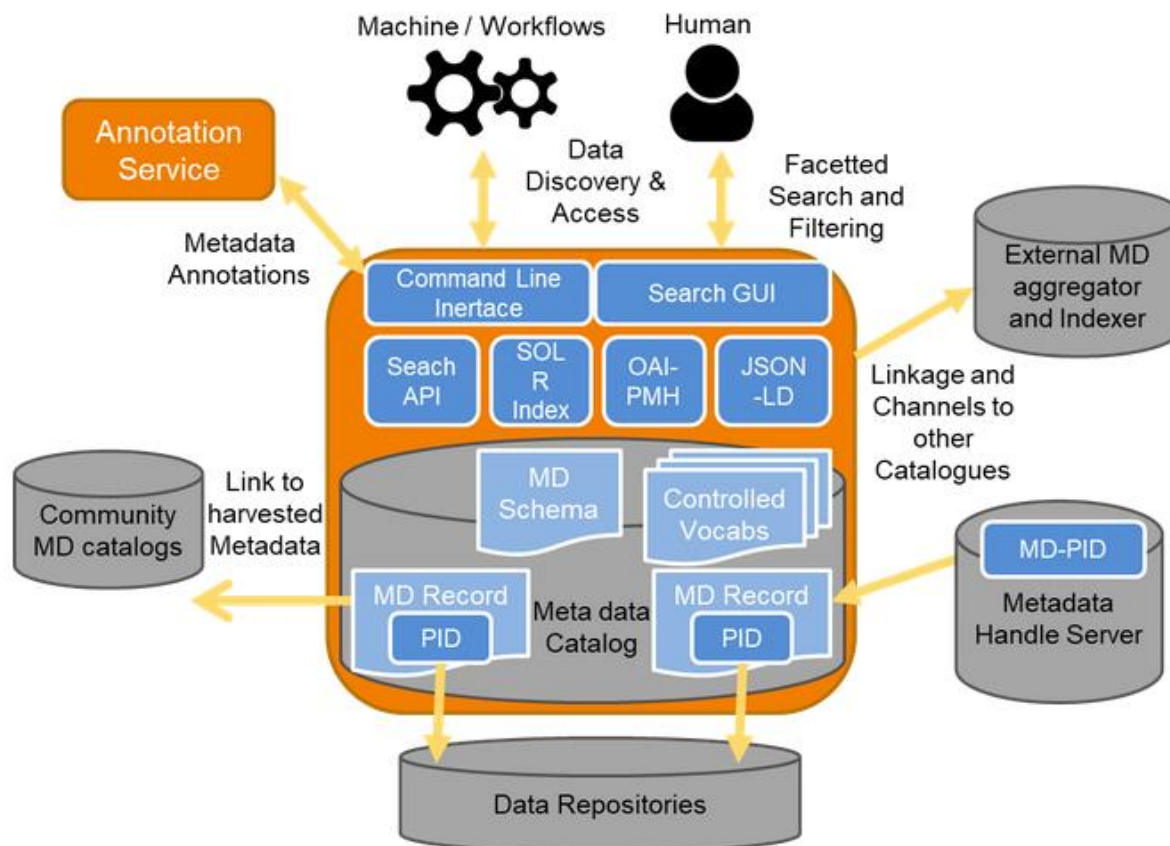
Figure 25: High level architecture diagram of Data Discovery and Access
