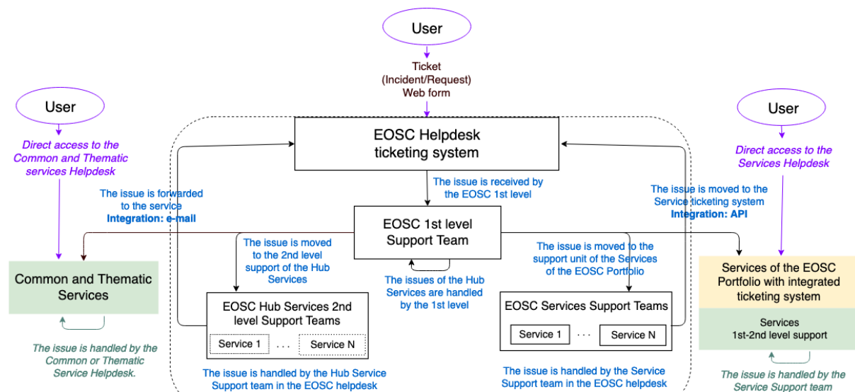
Fig. 3. High-level architecture of the EOSC Helpdesk
