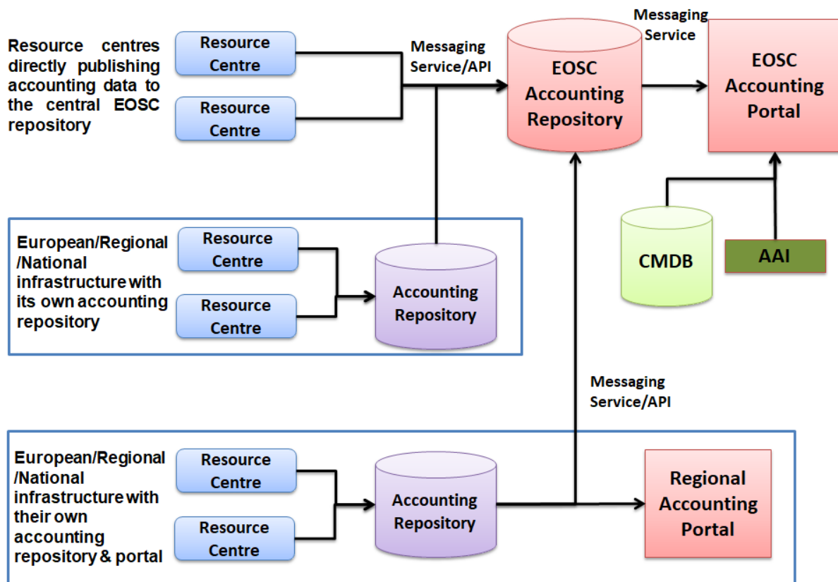
Fig. 2. High-level architecture of the EOSC Accounting
