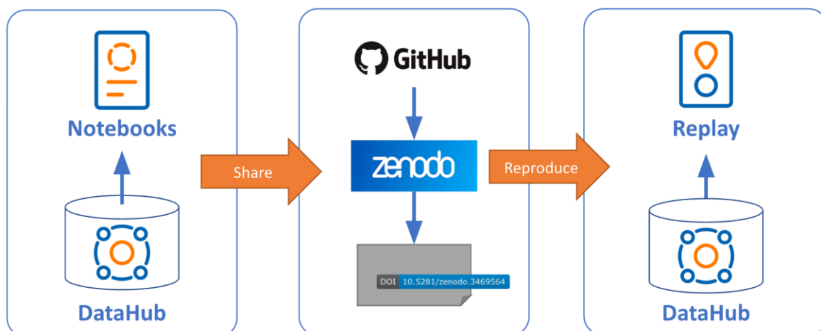
Figure 6.4 - Replay workflow
