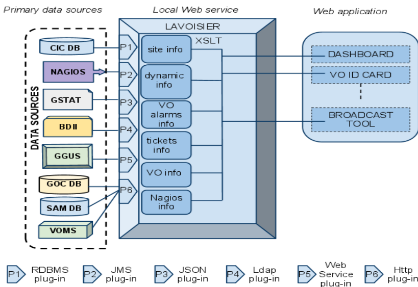
Figure 1: Global architecture of the Operations Portal.
