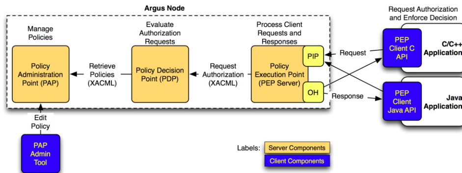
Fig. 2: Internal ARGUS Components
