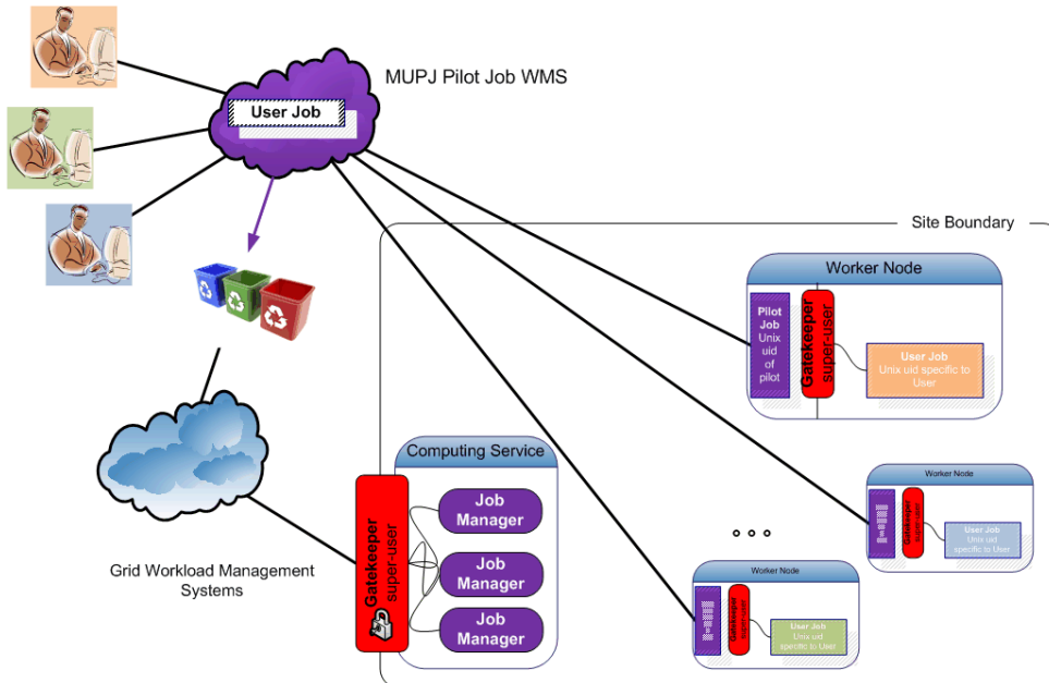
Fig. 1: gLExec and Argus integration
