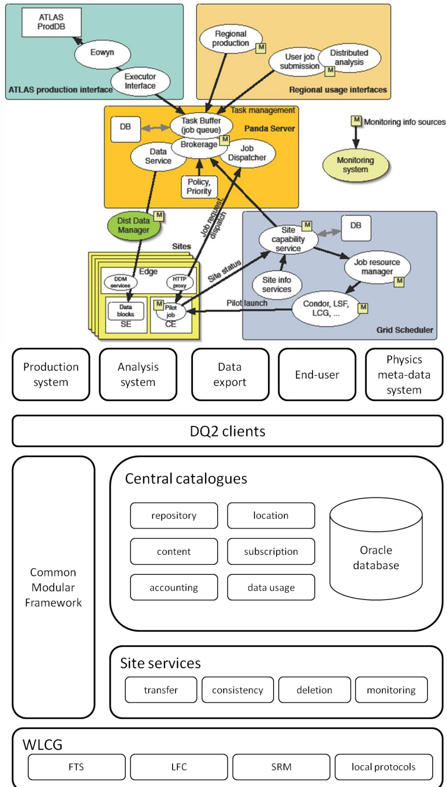
Figure 3. (a) PanDA architecture; (b) DDM architecture.
