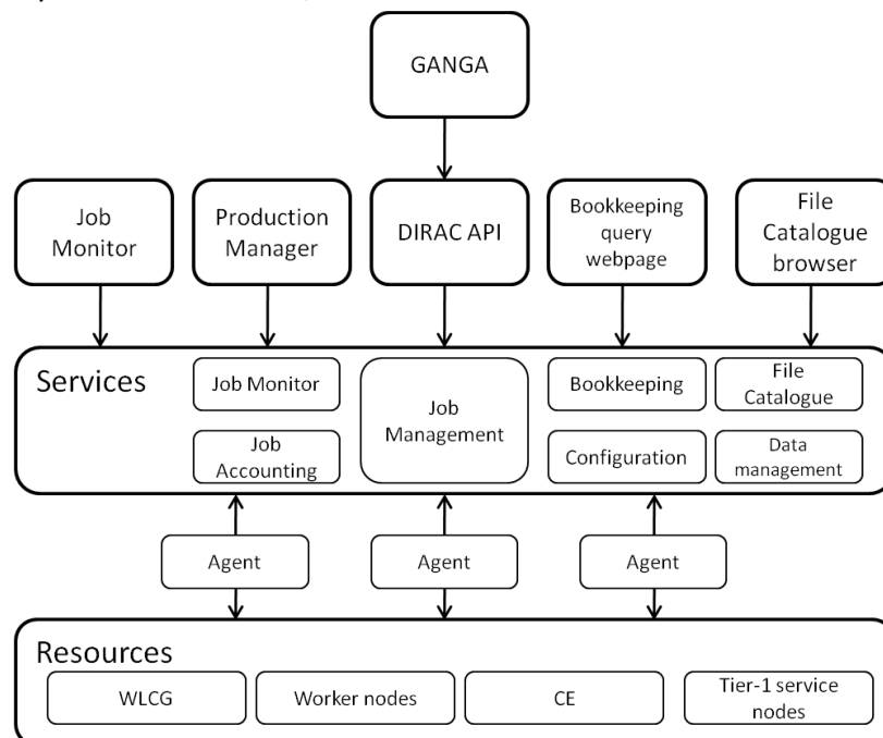
Figure 5. The DIRAC architecture.
